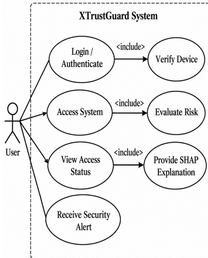
Figure 3.3: Use Case Diagram of XTrustGuard
