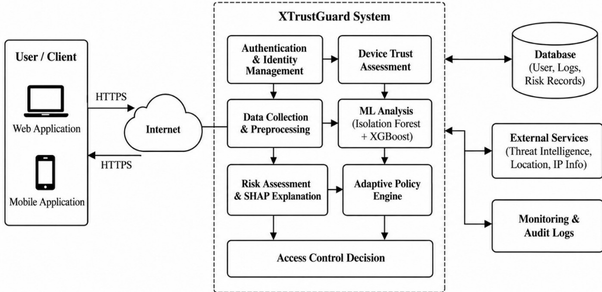
Figure 3.1: System Architecture of XTrustGuard
