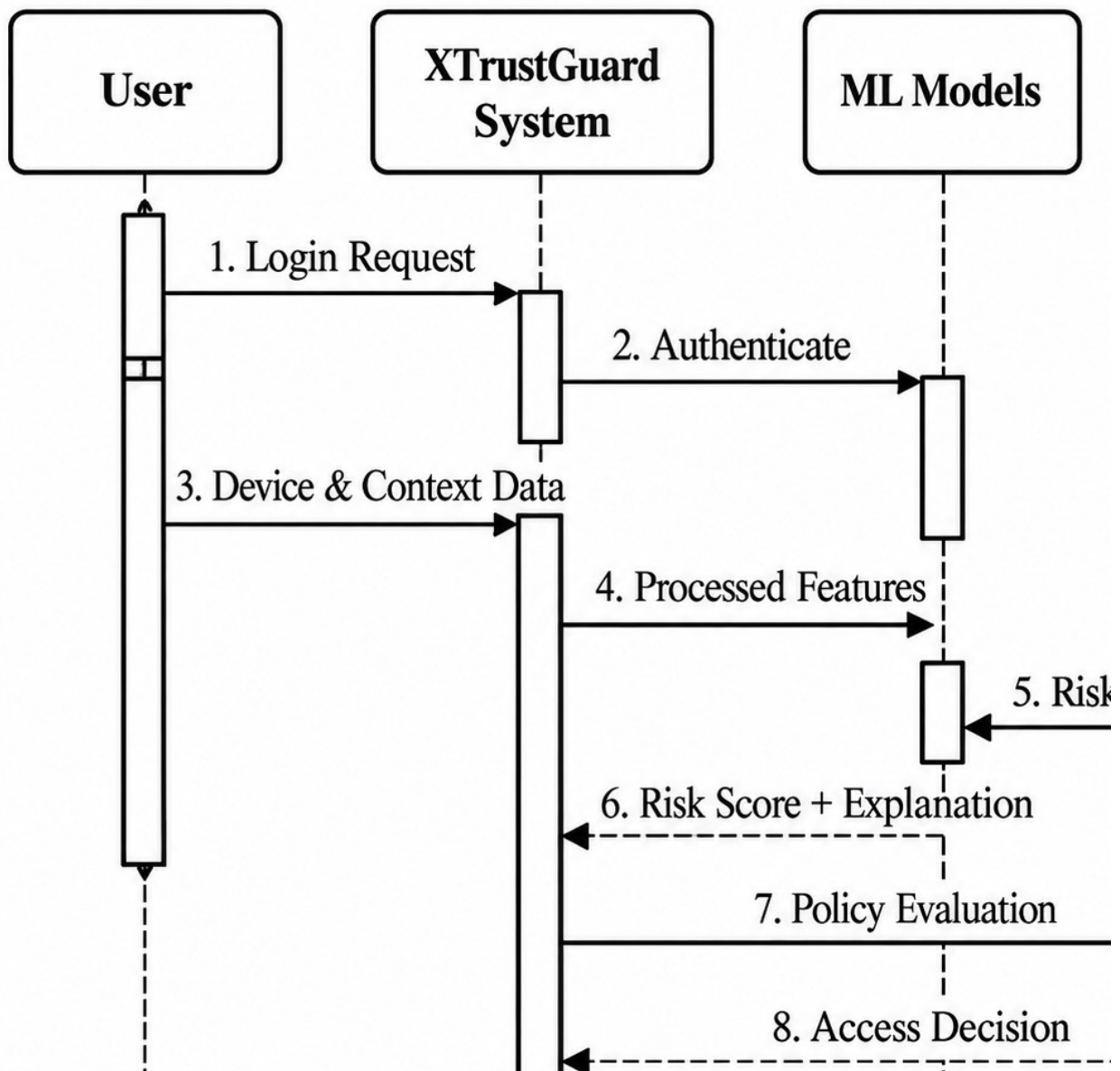
Figure 3.4: Sequence Diagram of XTrustGuard
