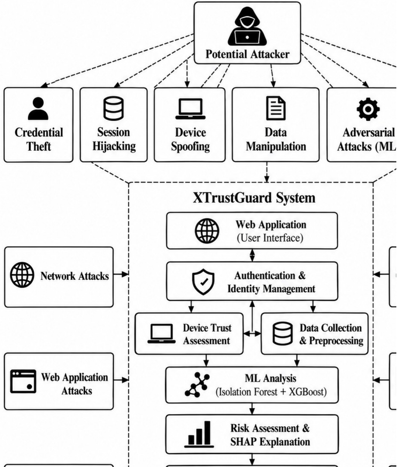
Figure 3.5: Threat Model and Attack Surface of XTrustGuard
